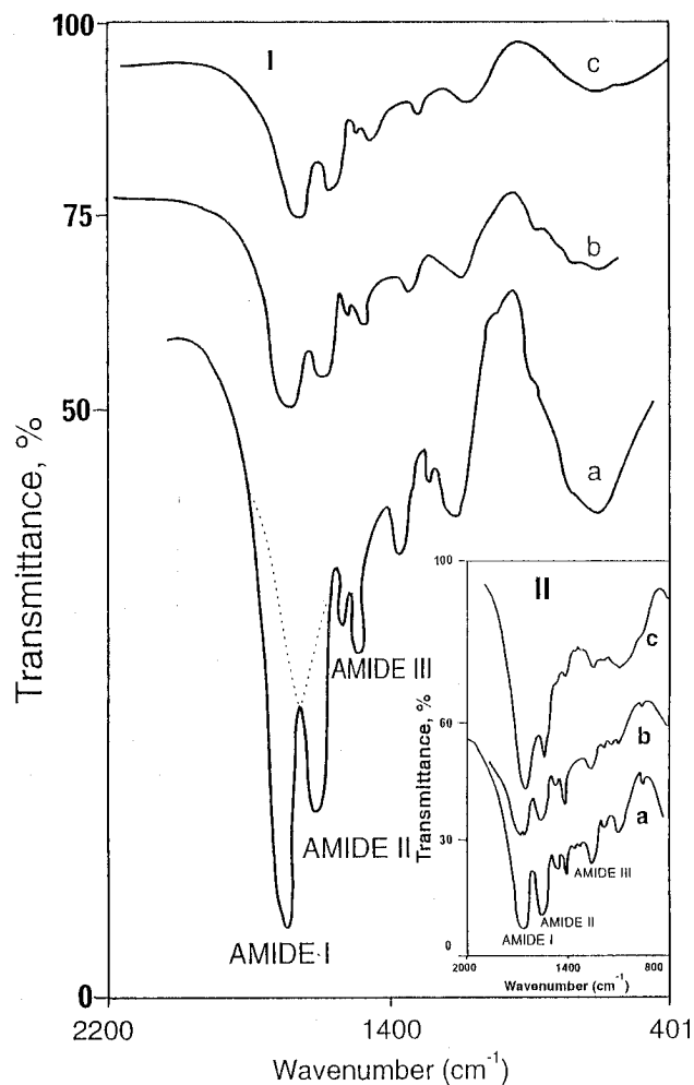
Figure 2. FT-IR spectra of A-G and \gamma -G: (section I) a = A-G, b = A-G at 100 °C, and c = A-G + GuHCl (1:1); (section II) a = \gamma -G, b = \gamma -G at 100 °C, and c = \gamma -G + GuHCl (1:1).
