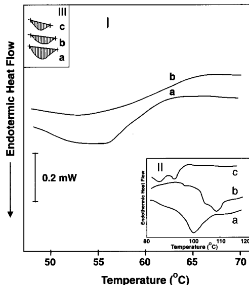
Figure 1. DSC thermograms of native and denaturated proteins: (section I) amaranth (A-S) and quinoa (Q-S) salt-soluble proteins, where a = A-S and b = Q-S; (section II) a = A-G with an average MW of 40 kDa, b = \gamma -G with a MW of 150 kDa, and c = A-G + 3 M urea; (section III) a = \gamma -G; b = \gamma -G at 100 °C; c = \gamma -G at 100 °C for 5 days.
