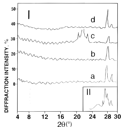
Figure 3. X-ray diffraction patterns of A-G and Q-G (section I) a = A-G, b = A-G at 100 °C, c = A-G + urea (1:1) and d = Q-G; (section II) urea.
