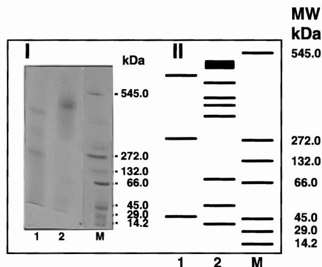
Figure 4. PAGE of native A-G in 8–25% PAAG: (section I) 1 = A-G; 2 = A-G at 100 °C; and M = marker; (section II) same conditions presented schematically.
